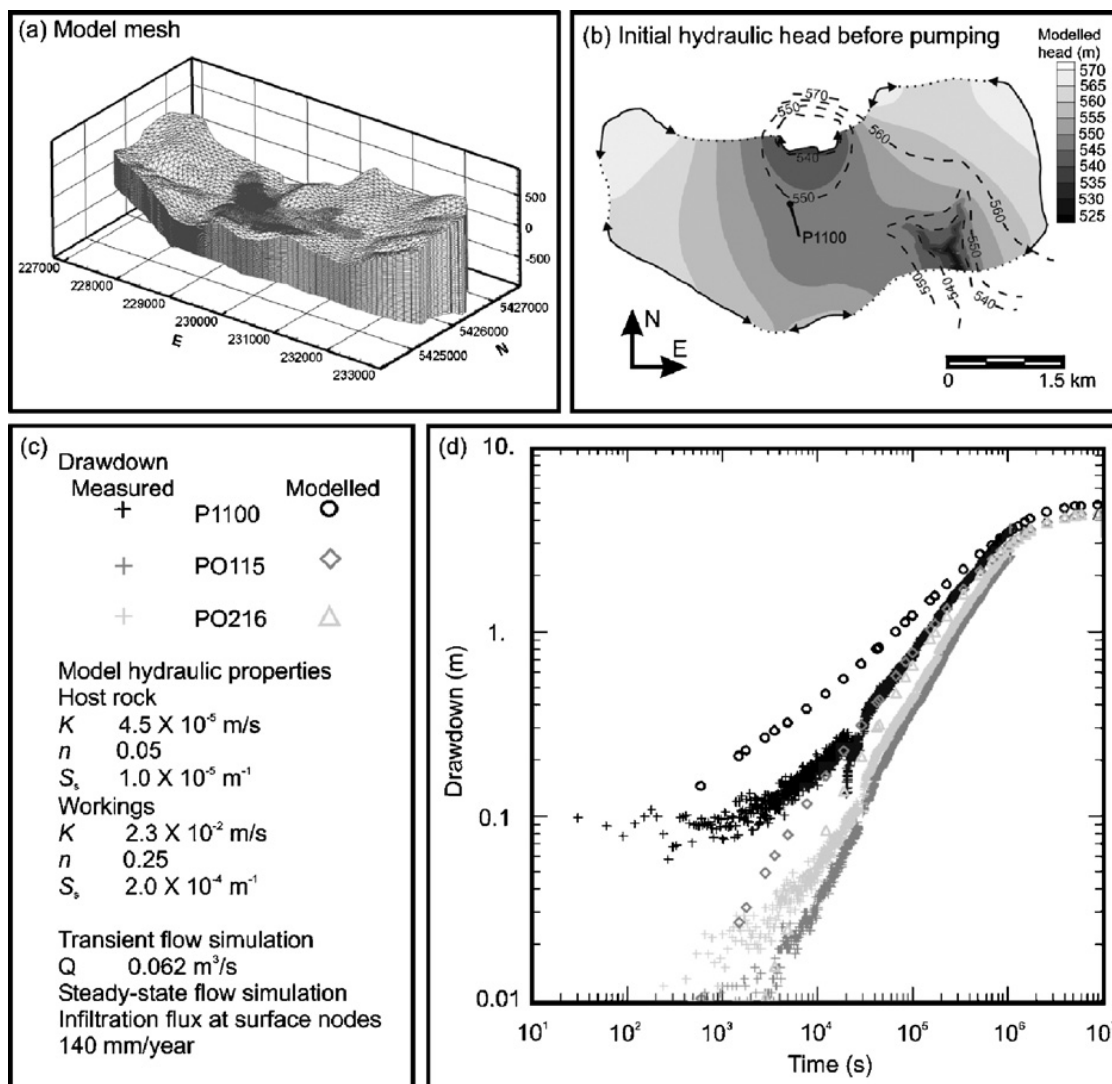
Fig. 7. Model mesh and simulation results obtained during model calibration. (a) Coordinate system (in m) used is the Modified Transverse Mercator NAD83. Legend on the vertical axis shows elevations (masl). (b) The initial hydraulic heads before pumping shown in plan view were obtained by steady-state fluid flow simulation. The constant head (solid lines with arrows) and impermeable boundaries (dotted lines) and the measured water table elevation (dashed lines) are shown with simulation results. Black dot corresponds to the location of shaft P1100 at ground surface. (c) Model hydraulic properties. (d) Modelled drawdown obtained by transient flow simulation.
