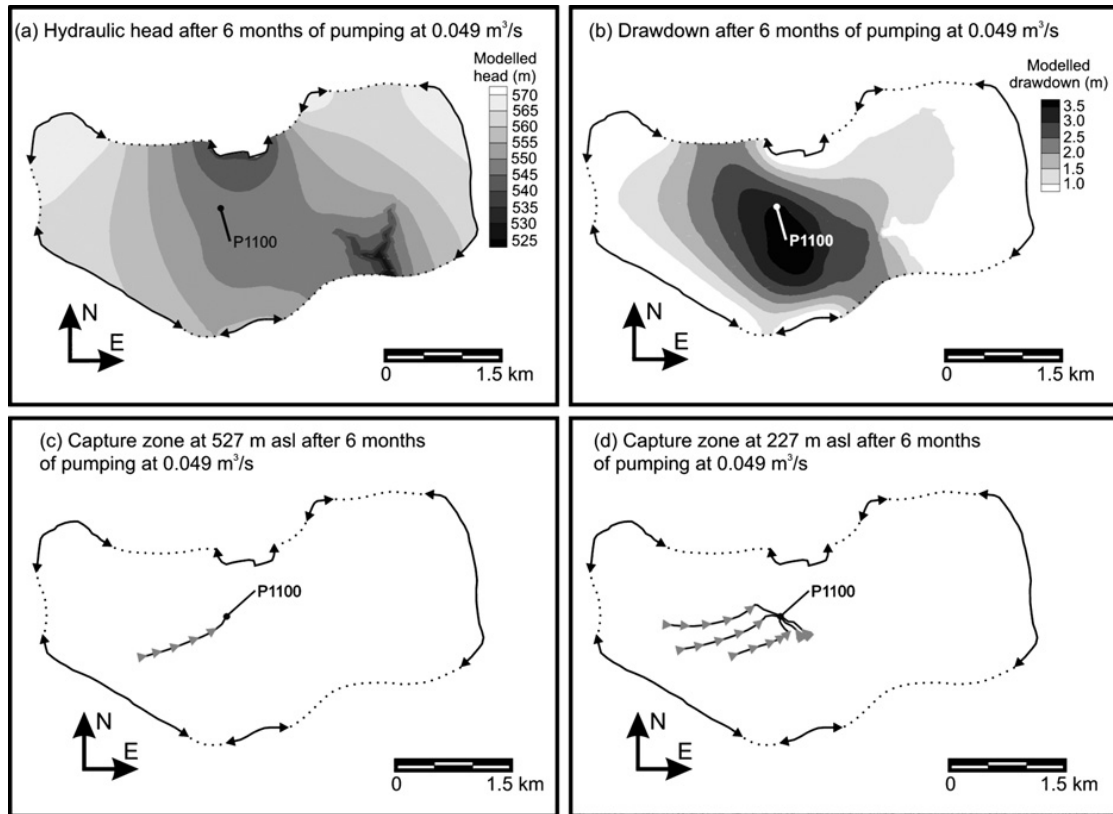
Fig. 8. (a) Modelled hydraulic head, (b) drawdown, and (c and d) capture zones shown in plan view at two different elevations after 6 months of pumping at a rate of 0.049 m³/s (2940 L/m). Grey triangles in the capture zones are placed at 10-year travel-time intervals. Dots representing shaft P1100 correspond to its location at surface in (a) and (b) and to its location at the elevation of the capture zone in (c) and (d). Constant head (solid lines with arrows) and impermeable boundaries (dotted lines) are shown on the maps.
